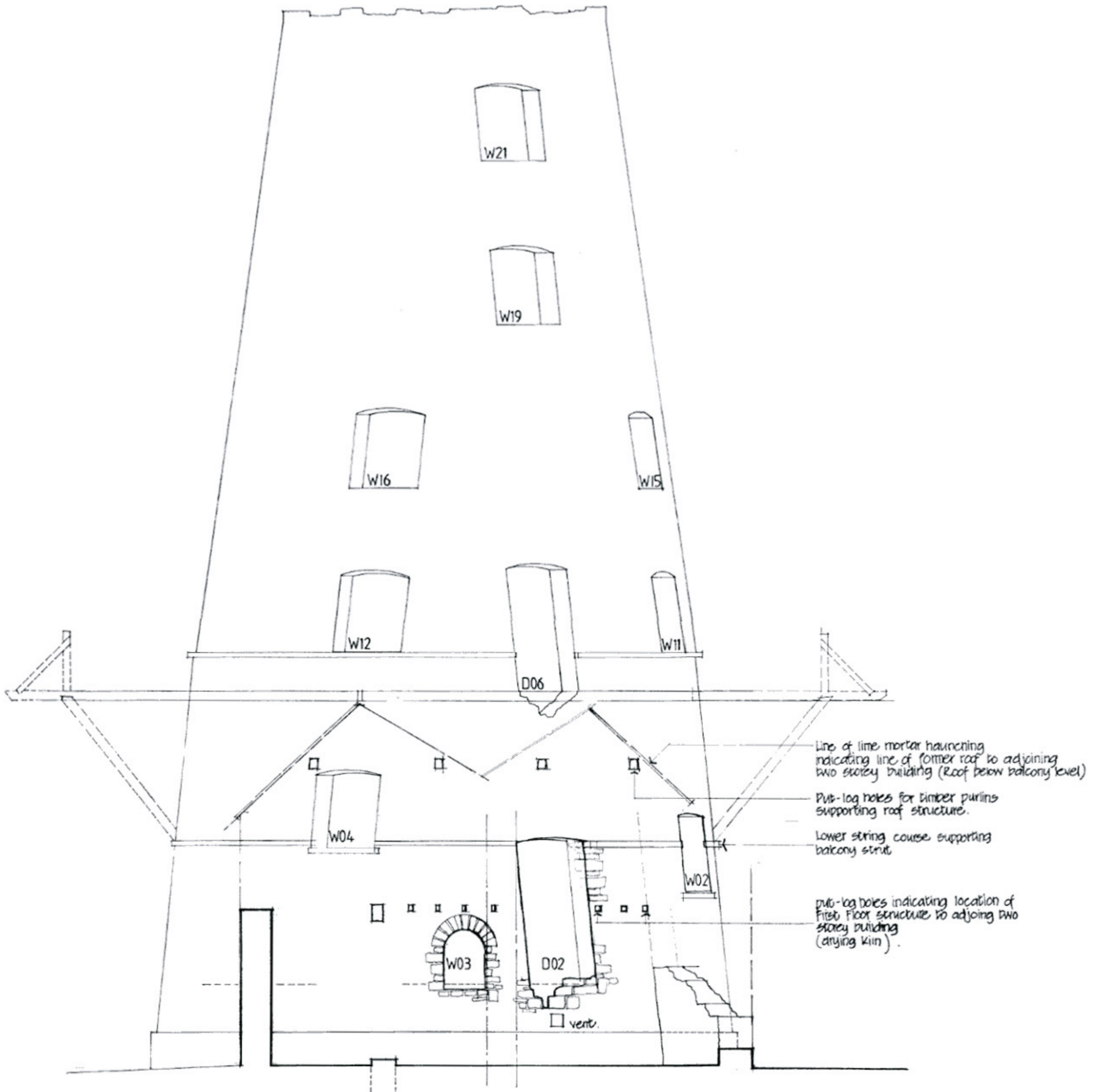
SECTION BB (indicating roof line of adjoining two storey building). North Facing Elevation.
