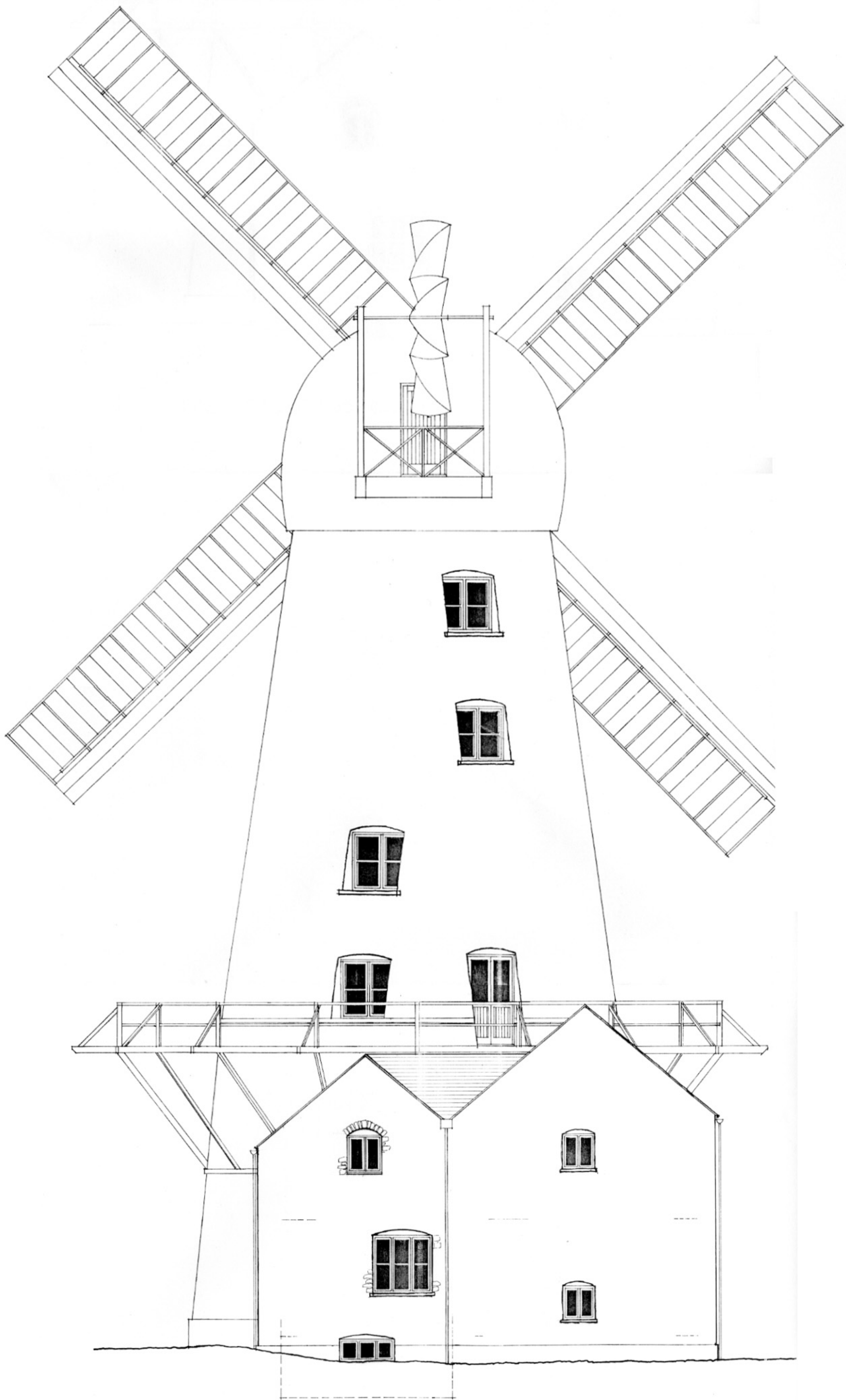
NORTH ELEVATION AS PROPOSED
