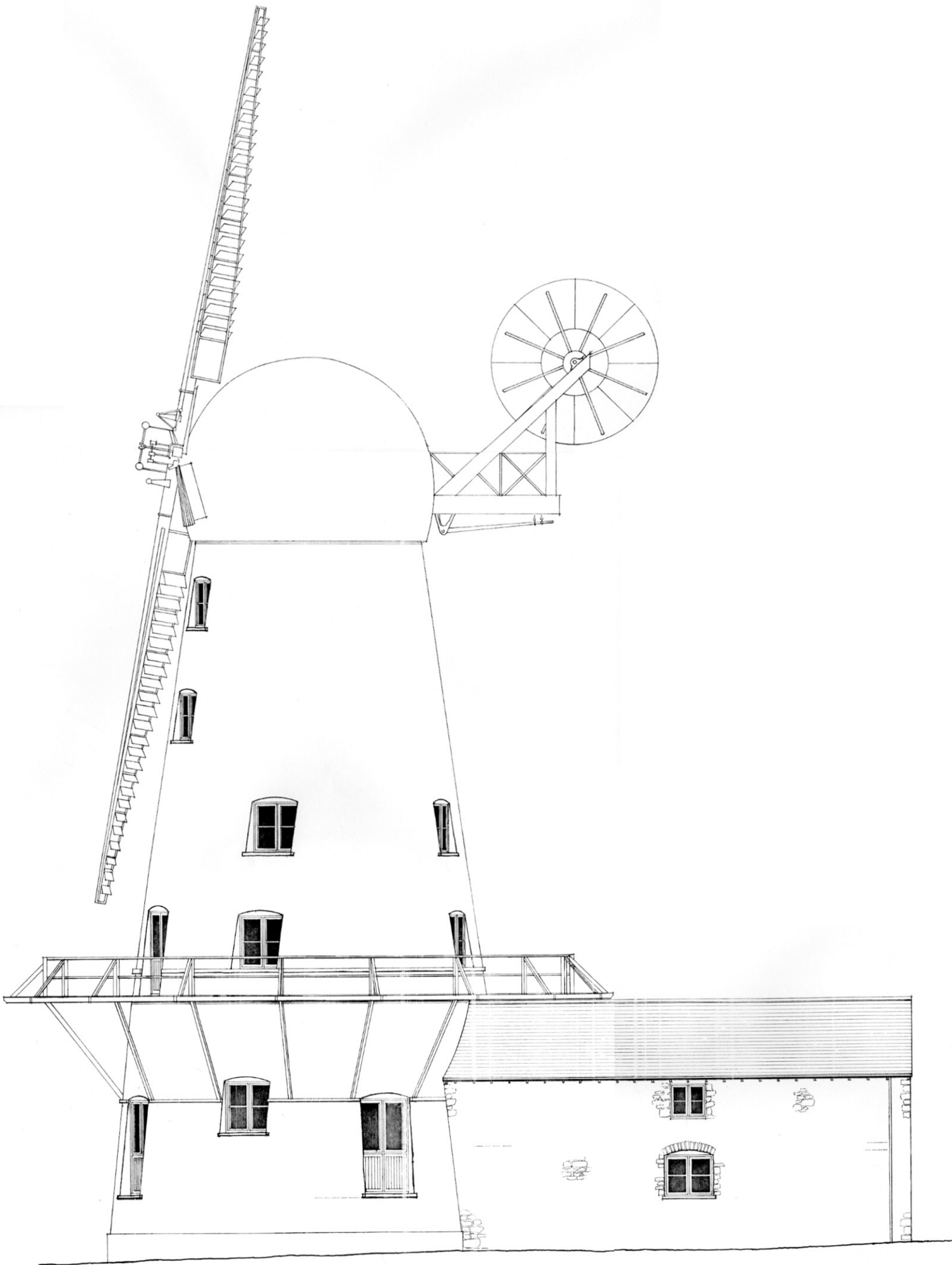
EAST ELEVATION AS PROPOSED
