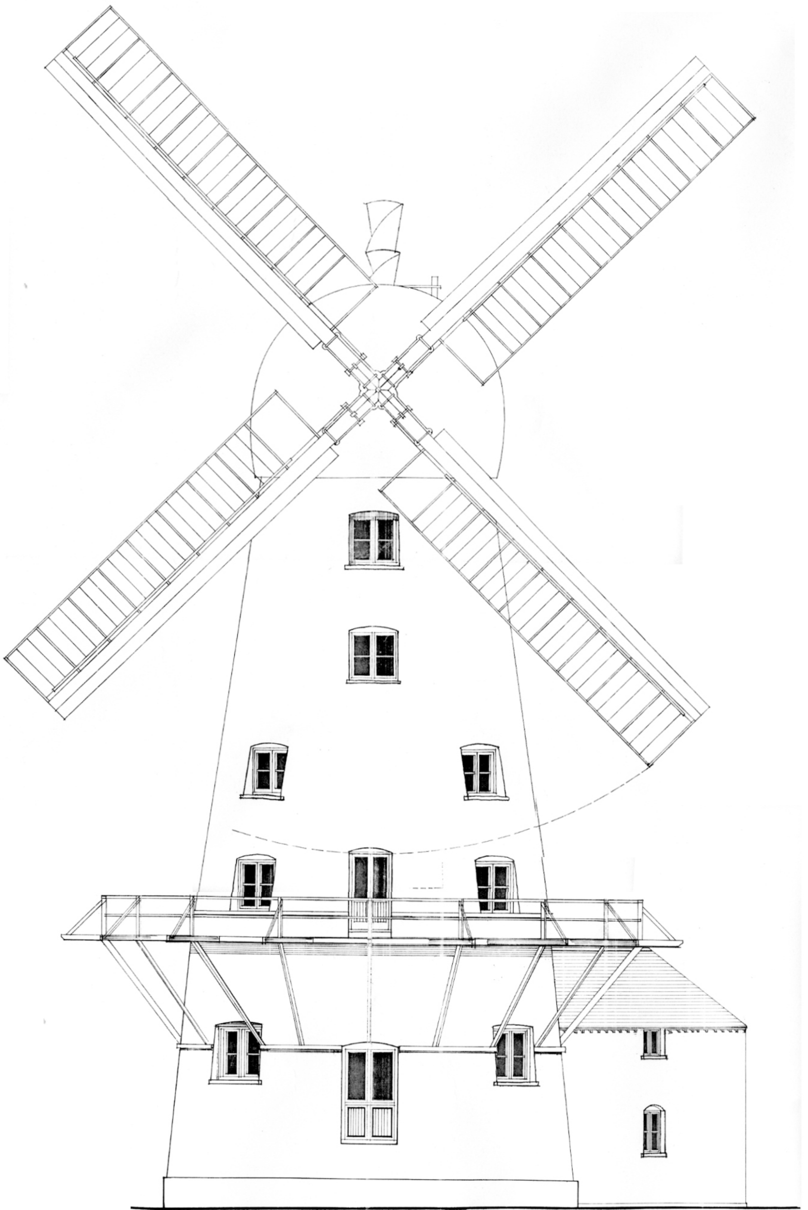
SOUTH EAST ELEVATION AS PROPOSED
