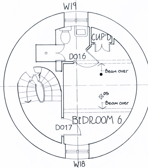
THIRD FLOOR PLAN (Level D)
