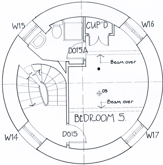
SECOND FLOOR PLAN (Level C)
